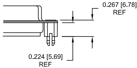
90X ..... 0.237" BOARD SIDE
