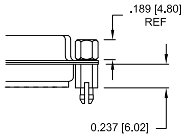
92X ..... 0.237" BOARD SIDE 0.189 MATING SIDE
