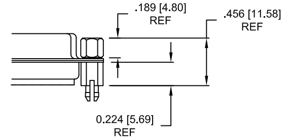
91X ..... 0.224" BOARD SIDE 0.189 MATING SIDE
