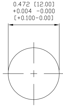
PANEL CUTOUT
