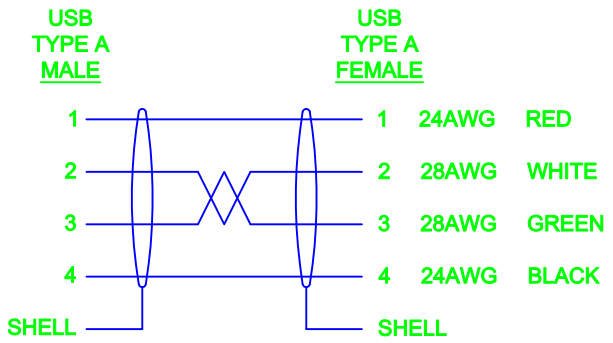
MALE-TO-FEMALE PINOUT
