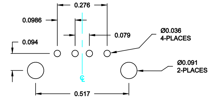
RECOMMENDED PCB LAYOUT SCALE = 3 : 1
