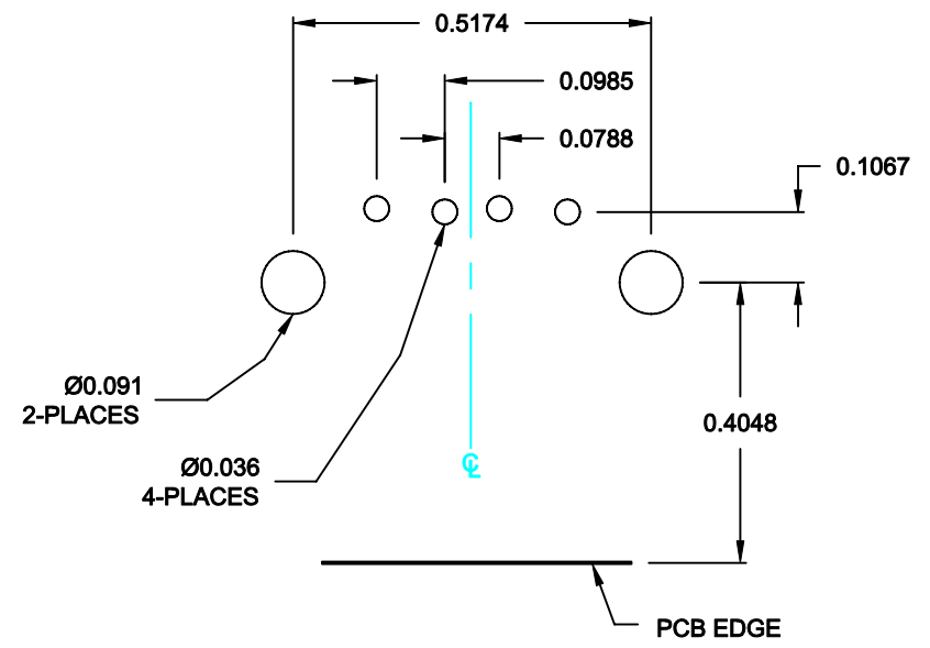
RECOMMENDED PCB LAYOUT SCALE = 3 : 1
